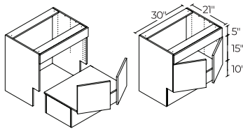
2 DOORS 30" | VS30FFRFADA
