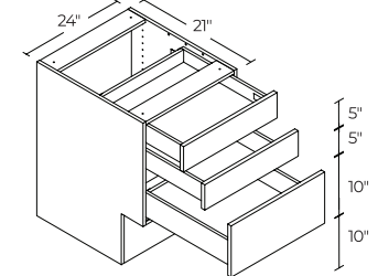
3 DRAWERS 24" | V3D24ADA
