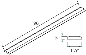
SCRIBE MOULDING
