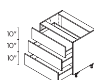
3 DRAWERS 36" | BCT3D36A
