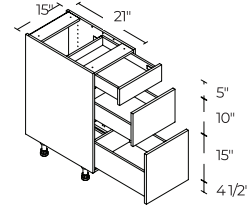
3 DRAWERS 15" | V3D15
