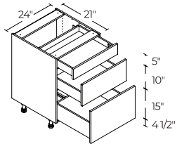
3 DRAWERS 24" | V3D24
