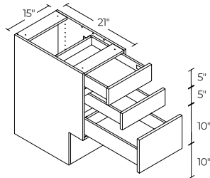
3 DRAWERS 15" | V3D15ADA
