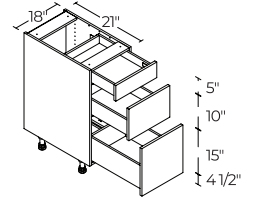
3 DRAWERS 18" | V3D18
