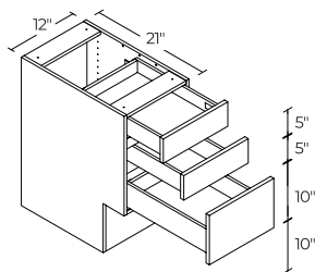
3 DRAWERS 12" | V3D12ADA
