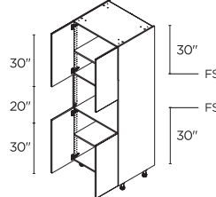
MICROWAVE 1 4 DOORS
