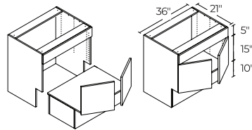
2 DOORS 36" | VS36FFRFADA
