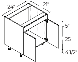
2 DOORS 24" | VS24
