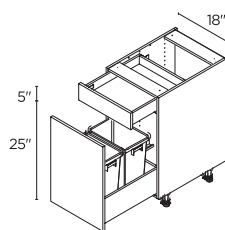
PULL-OUT / 1 DRAWER
