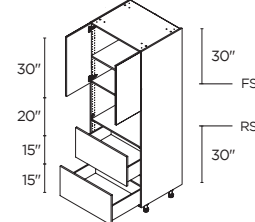
MICROWAVE 1 2 DOORS / 2 DRAWERS 30" | TM2D3084.5
