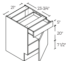
1 DOOR / 1 DRAWER 21" | B21ADA
