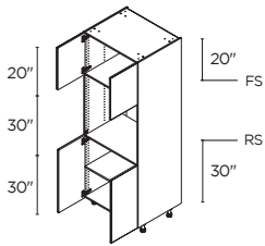
SINGLE OVEN 4 4 DOORS 30" | TO3084.5
