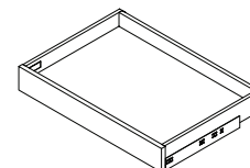
INNER DRAWER KIT 24" 12 x 3 3/8" | DK1224 15 x 3 3/8" | DK1524 18 x 3 3/8" | DK1824 21 x 3 3/8" | DK2124 24 x 3 3/8" | DK2424 27 x 3 3/8" | DK2724 30 x 3 3/8" | DK3024 33 x 3 3/8" | DK3324 36 x 3 3/8" | DK3624
