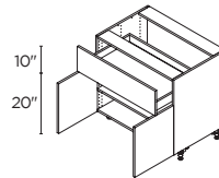
2 DOORS / 1 DRAWER 36" | BCT36A
