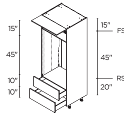
MICRO/WALL OVEN 2 1 LIFT-UP DOOR / 2 DRAWERS 30" | TMOL2DA3084.5
