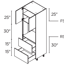
SINGLE OVEN 3 2 DOORS / 2 DRAWERS 30" | TO2D3089.5
