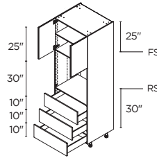
SINGLE OVEN 3 2 DOORS / 3 DRAWERS 30" | TO3DA3089.5
