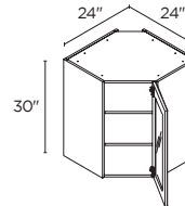
30" HIGH 1 GLASS DOOR*
