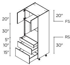
SINGLE OVEN 4 2 DOORS / 3 DRAWERS 30" | TO3D3084.5
