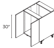
2 DOORS 24" | SB24-2FH 27" | SB27FH 30" | SB30FH 33" | SB33FH 36" | SB36FH
