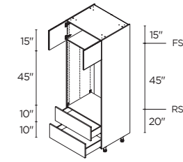
MICRO/WALL OVEN 2 2 DOORS / 2 DRAWERS 30" | TMO2DA3084.5
