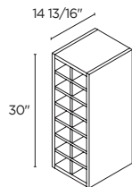
WALL WINE RACK
