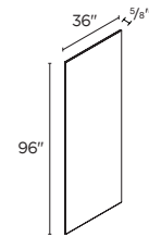
TALL CABINET & FRIDGE GABLE COVER PANEL 36"
