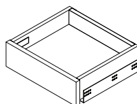
SHALLOW INNER DRAWER KIT 14" 15 x 3 3/8" | DK1514 18 x 3 3/8" | DK1814 24 x 3 3/8" | DK2414
