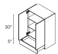
35" HIGH 2 DOORS / 1 DRAWER 24" | W2435-2A
