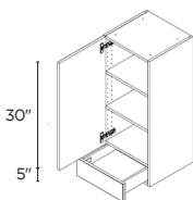
35" HIGH 1 DOOR / 1 DRAWER 15" | W1535A(L/R) 18" | W1835A(L/R) 24" | W2435A(L/R)
