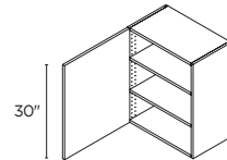
30" HIGH 1 DOOR 9" | W930(L/R) 18" | W1830(L/R) 12" | W1230(L/R) 21" | W2130(L/R) 15" | W1530(L/R) 24" | W2430(L/R)
