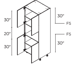
MICROWAVE 1 4 DOORS 30" | TM3084.5
