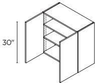
30" HIGH 2 DOORS 24" | W2430-2 27" | W2730 30" | W3030 33" | W3330 36" | W3630
