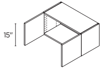
15" HIGH 2 DOORS 27" | W2715 30" | W3015 33" | W3315 36" | W3615
