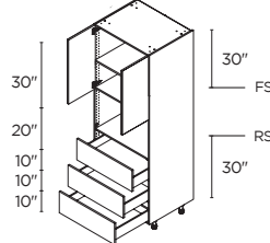
MICROWAVE 1 2 DOORS / 3 DRAWERS 30" | TM3DA3084.5
