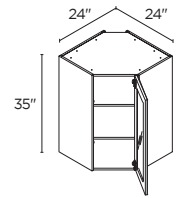
35" HIGH 1 GLASS DOOR*
