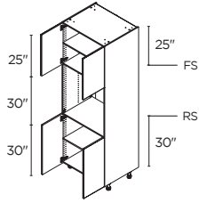
SINGLE OVEN 3 4 DOORS 30" | TO3089.5
