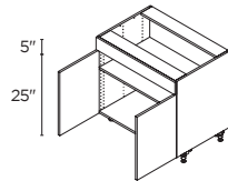
2 DOORS / 1 FIXED FRONT 36" | BCT36FF
