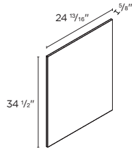
BASE CABINET COVER PANEL
