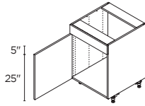
1 DOOR / 1 FIXED FRONT 24" | SB24FF(L/R)
