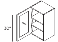
30" HIGH 1 GLASS DOOR* 15" | WG1530(L/R) 18" | WG1830(L/R)
