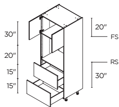
MICROWAVE 1 2 DOORS / 2 DRAWERS 30" | TM2D3084.5
