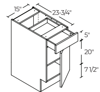
1 DOOR / 1 DRAWER 15" | B15ADA
