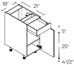
1 DOOR / 1 DRAWER 18" | V18(L/R)
